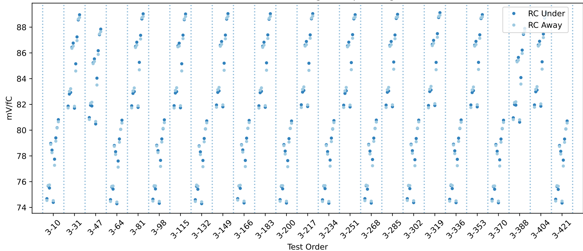
20USBHX2002957 RC gain chip averages
