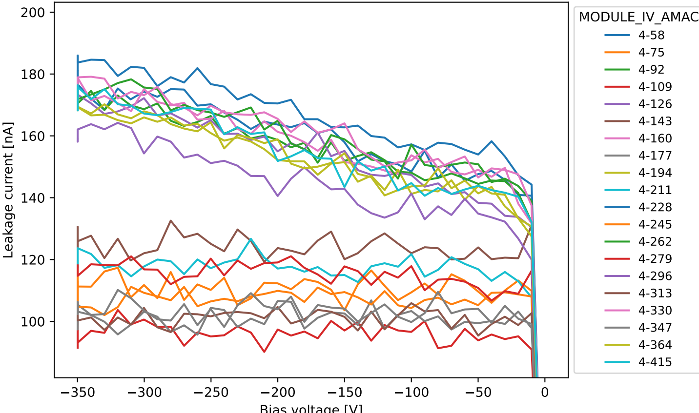
20USBML1236160 fast IV
