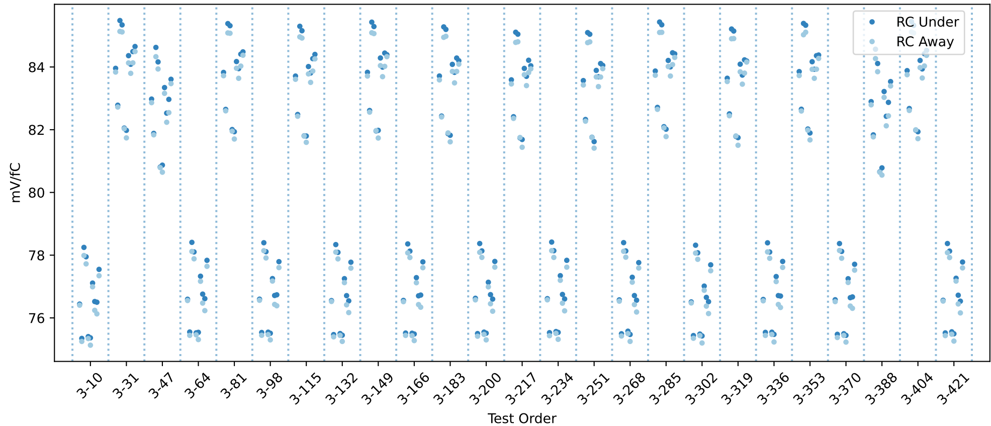
20USBHX2001815 RC gain chip averages
