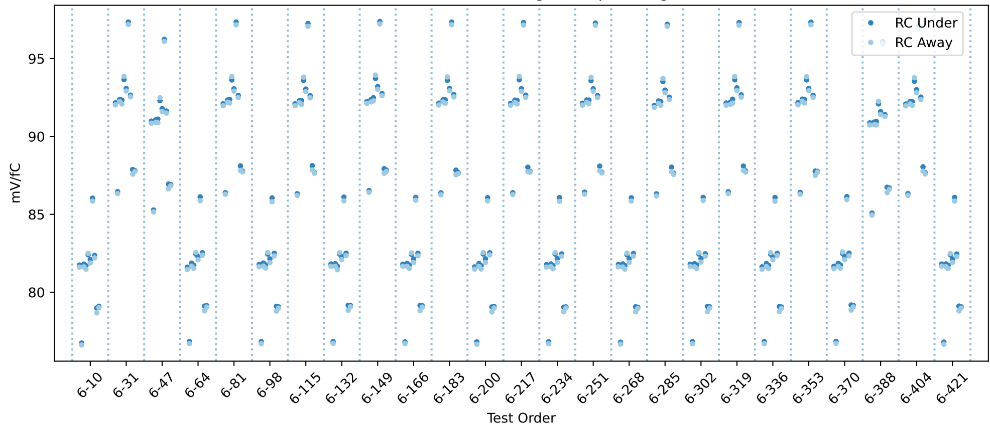
20USBHX2004003 RC gain chip averages
