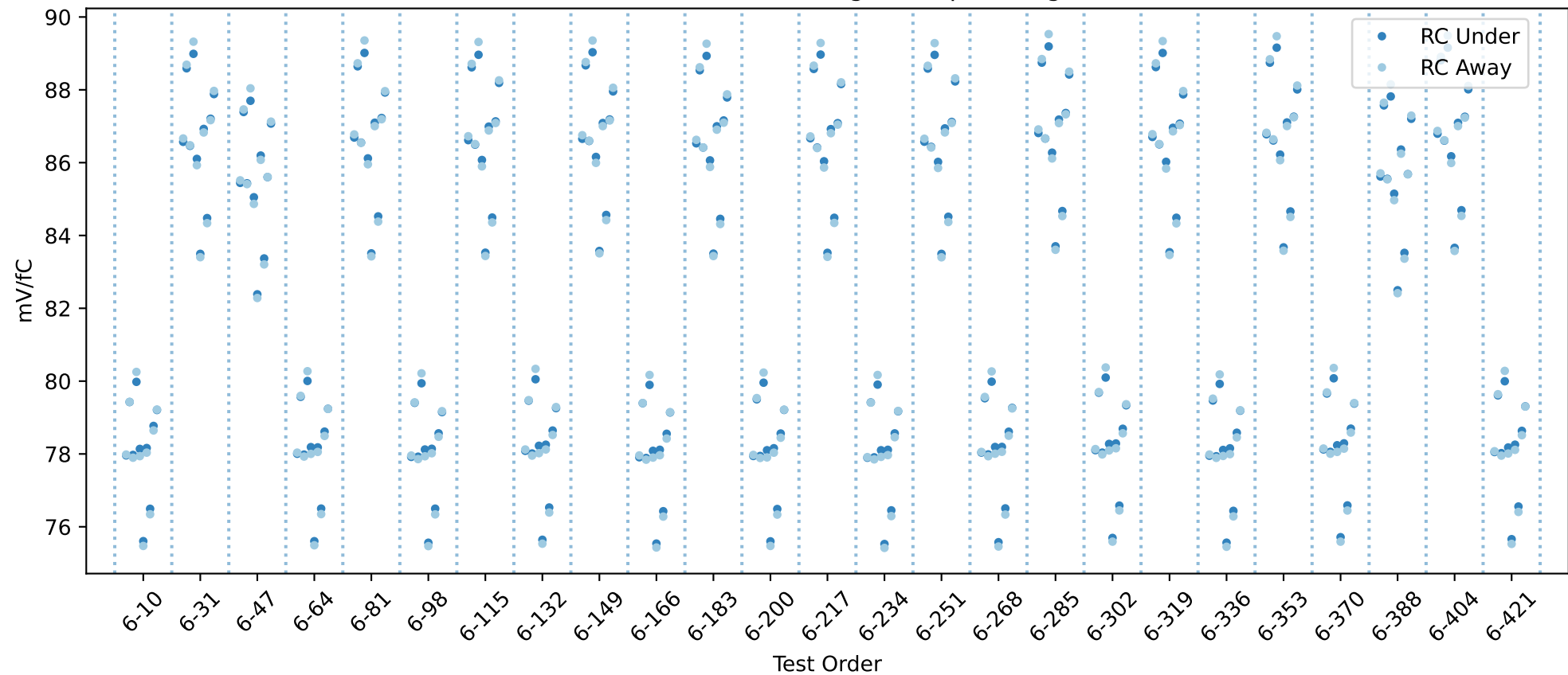
20USBHX2002640 RC gain chip averages
