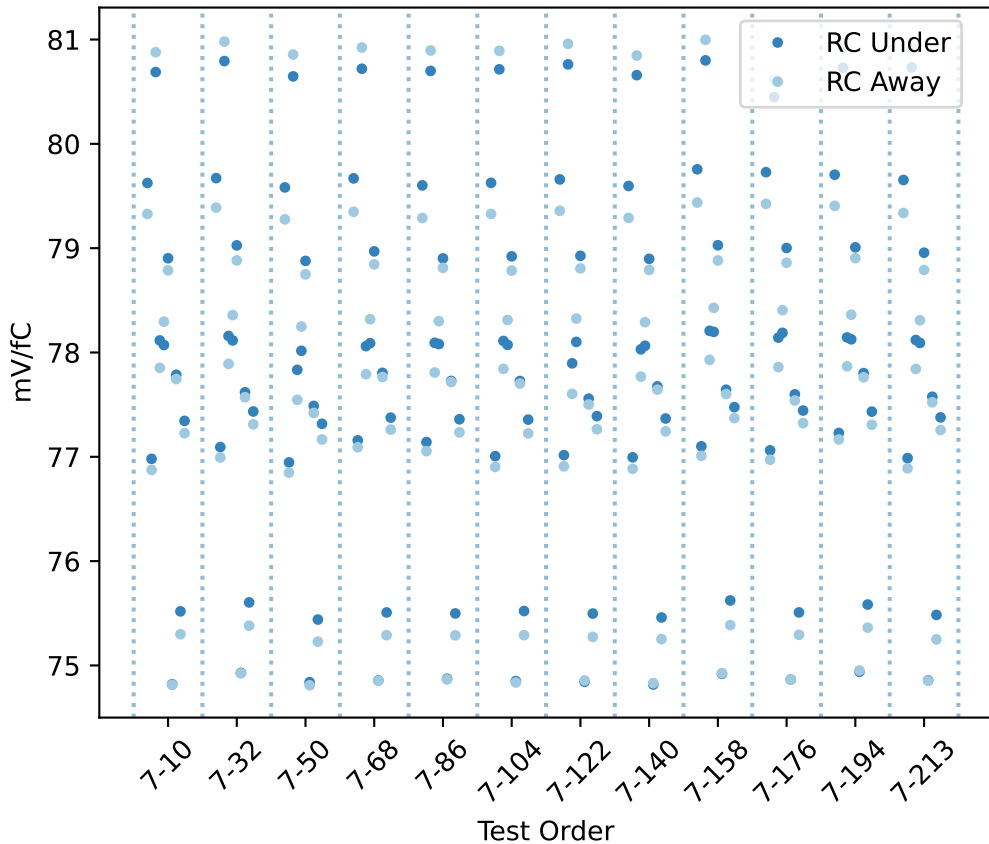
20USBHX2002646 RC gain chip averages
