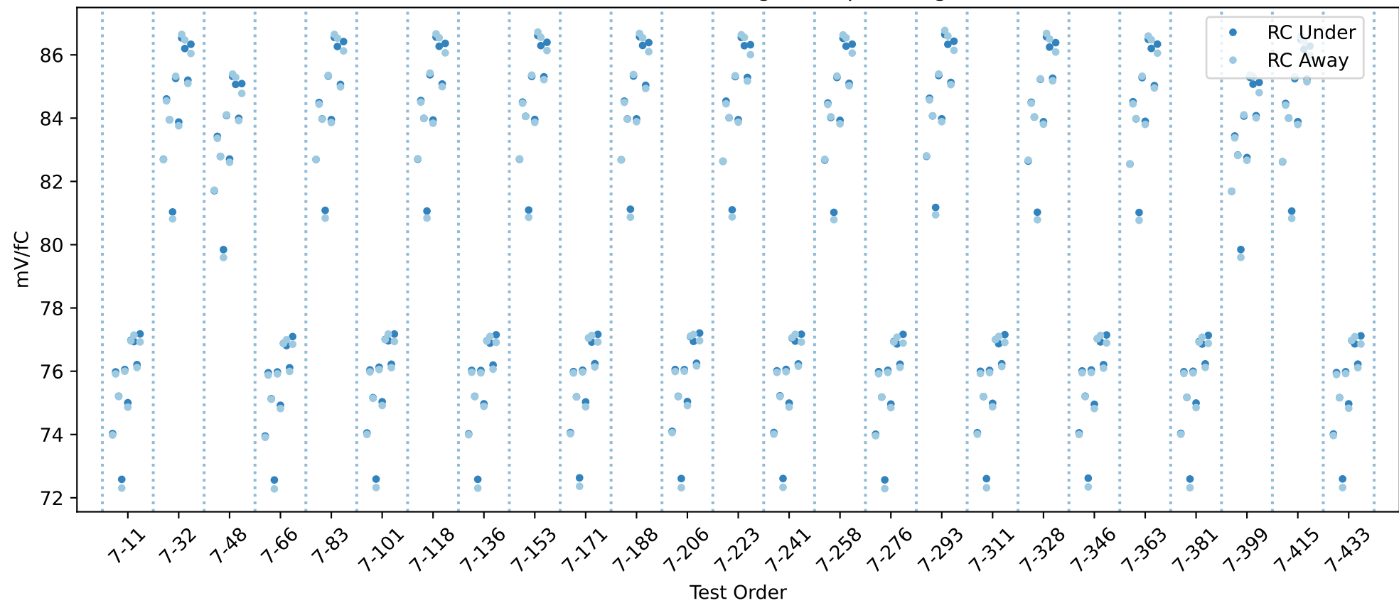
20USBHX2003075 RC gain chip averages
