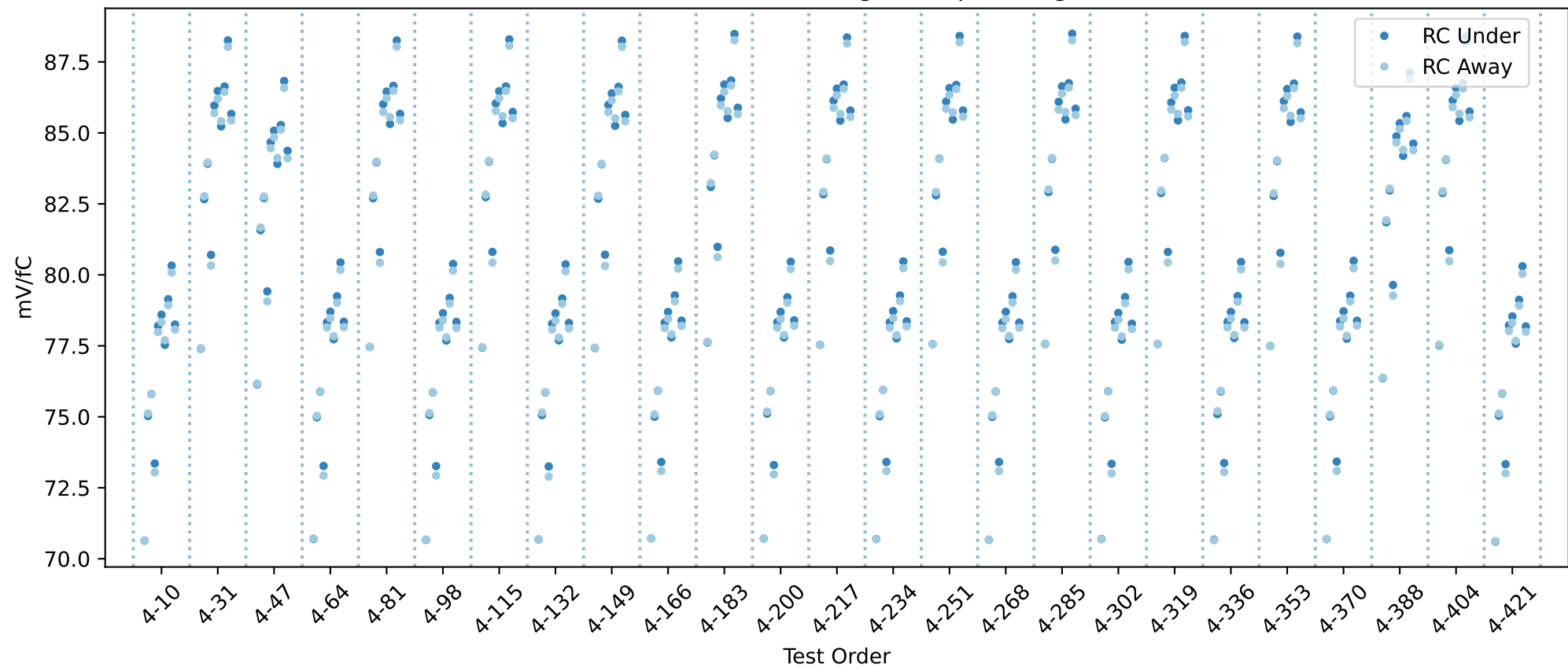
20USBHX2003412 RC gain chip averages
