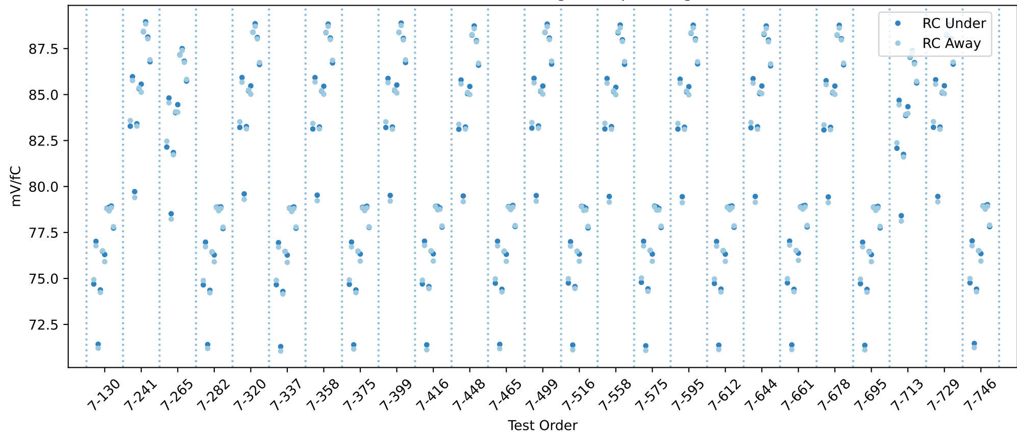
20USBHX2003281 RC gain chip averages
