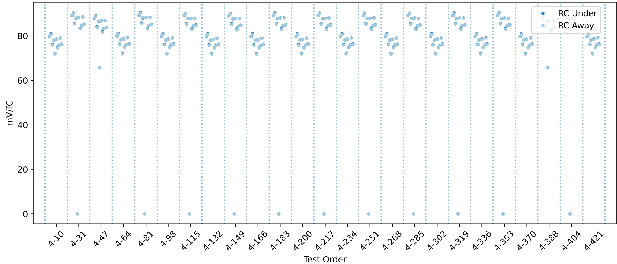
20USBHX2002283 RC gain chip averages
