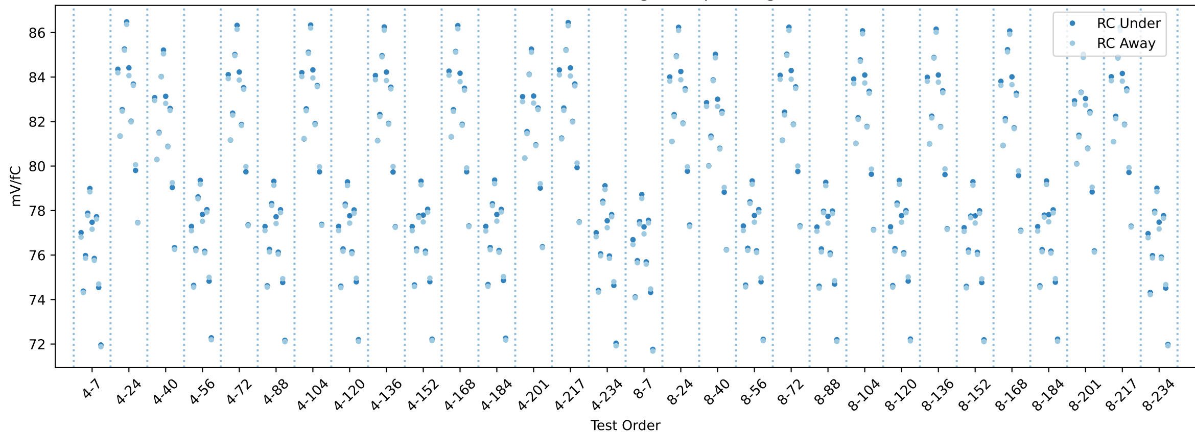
20USBHX2001388 RC gain chip averages
