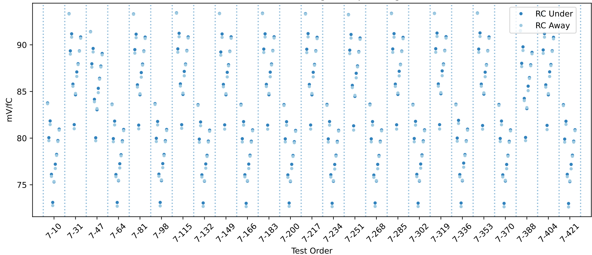
20USBHX2001398 RC gain chip averages
