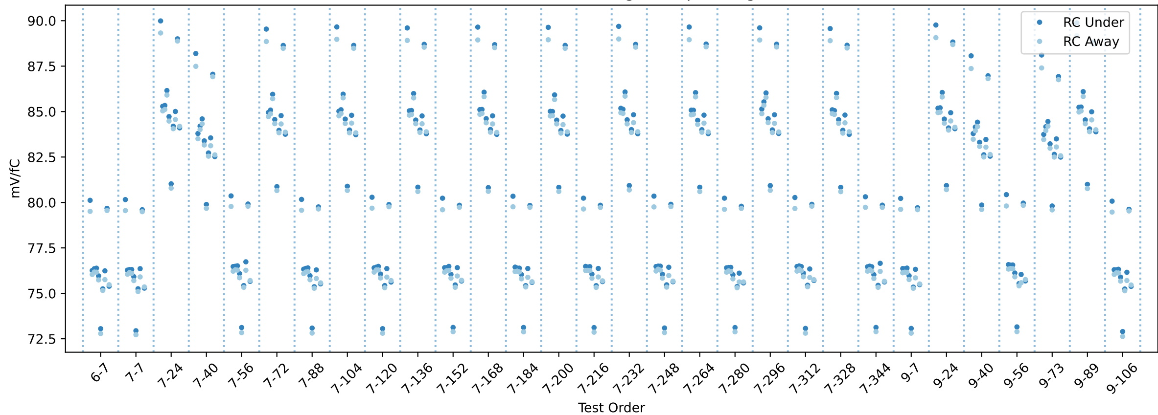
20USBHX2001479 RC gain chip averages
