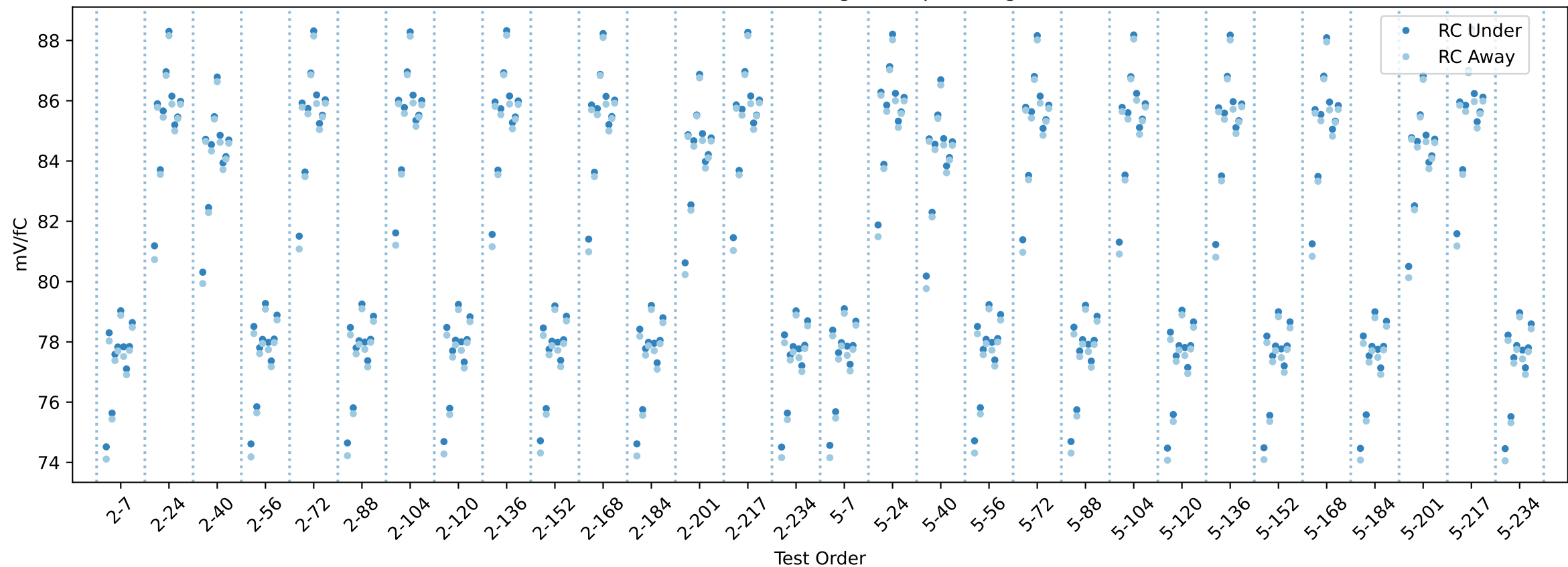
20USBHX2001490 RC gain chip averages
