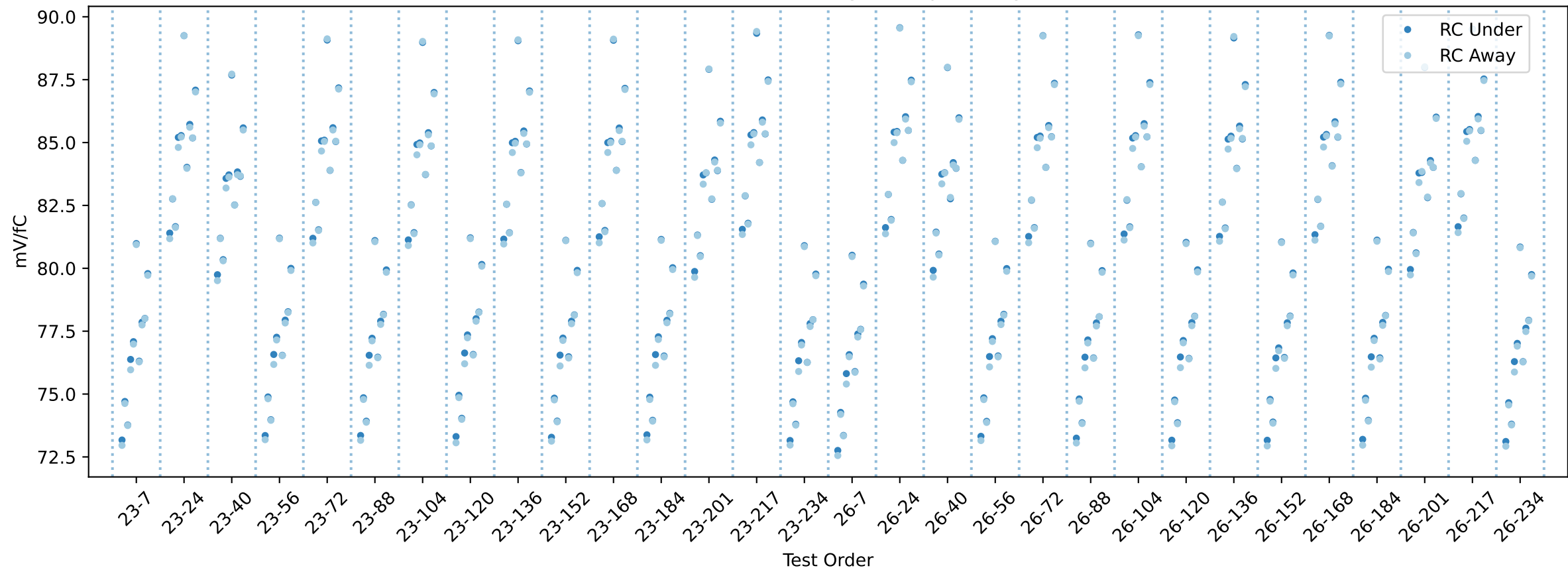
20USBHX2001482 RC gain chip averages
