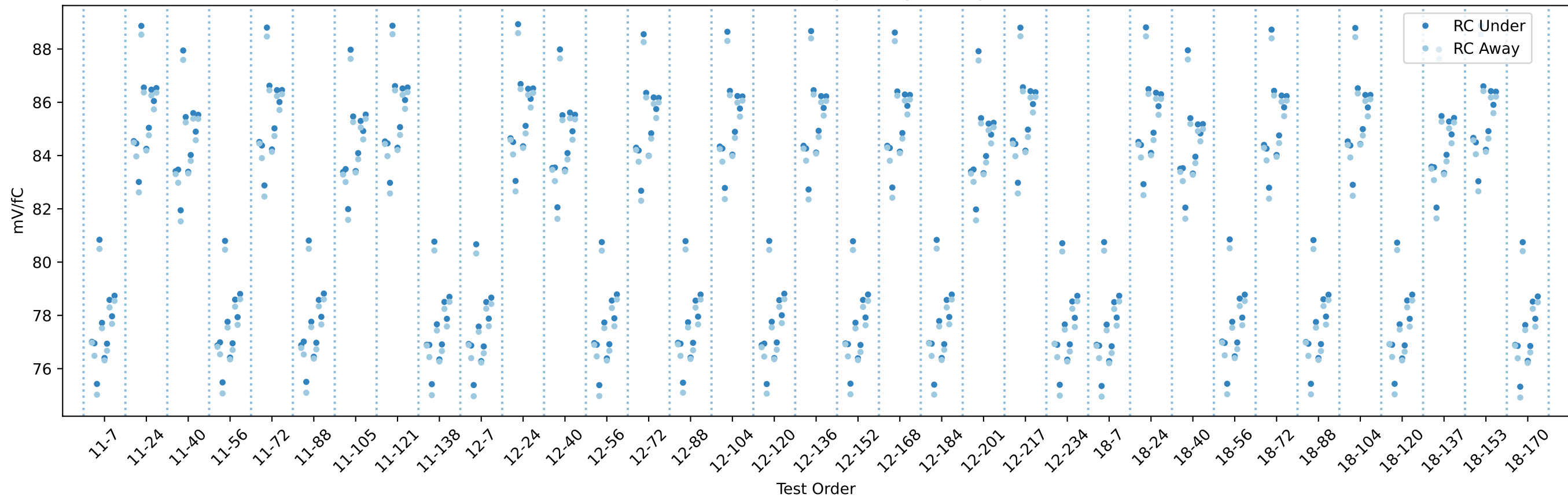
20USBHX2001761 RC gain chip averages
