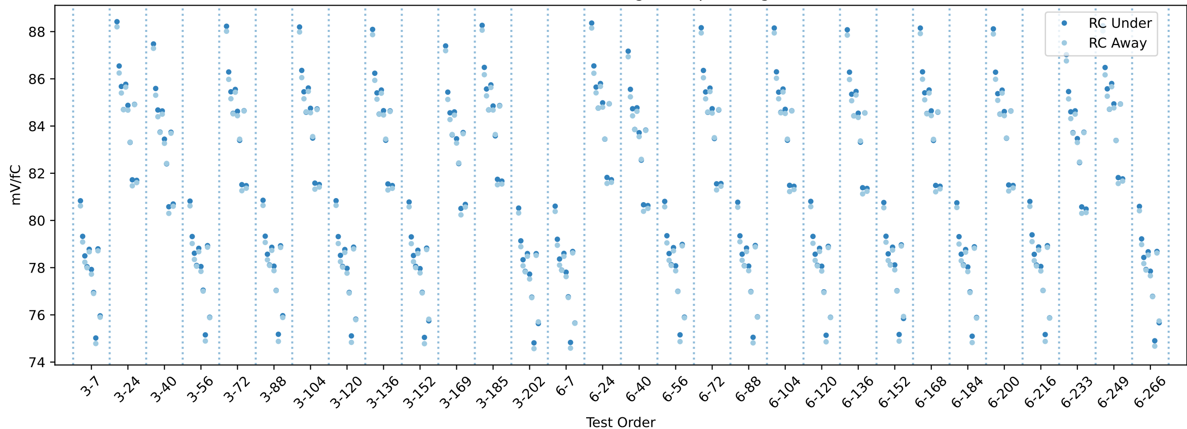
20USBHX2001804 RC gain chip averages
