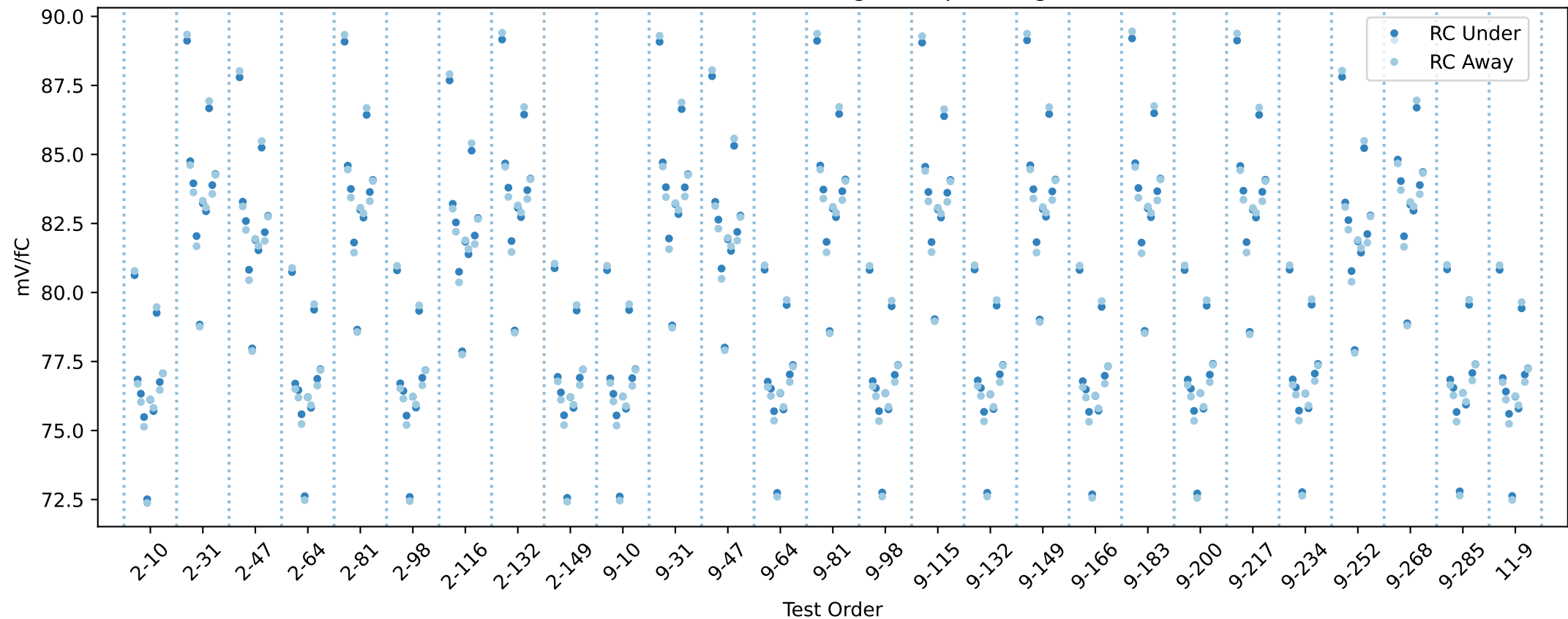
20USBHX2001429 RC gain chip averages
