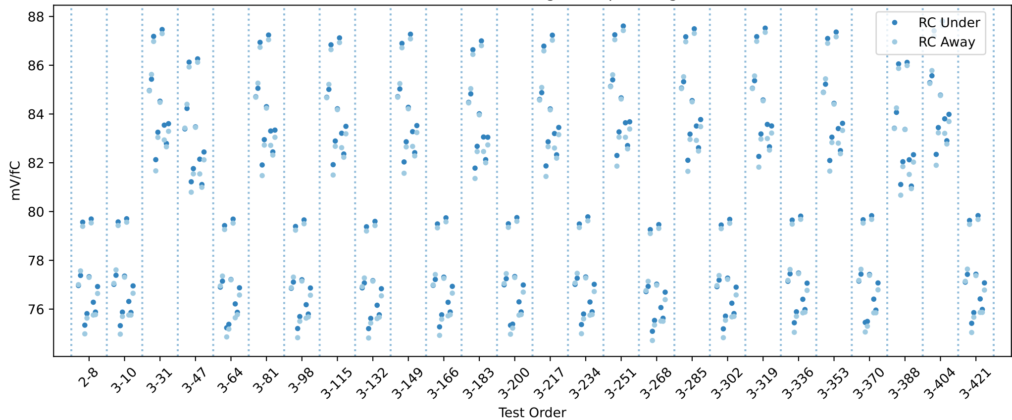
20USBHX2001888 RC gain chip averages
