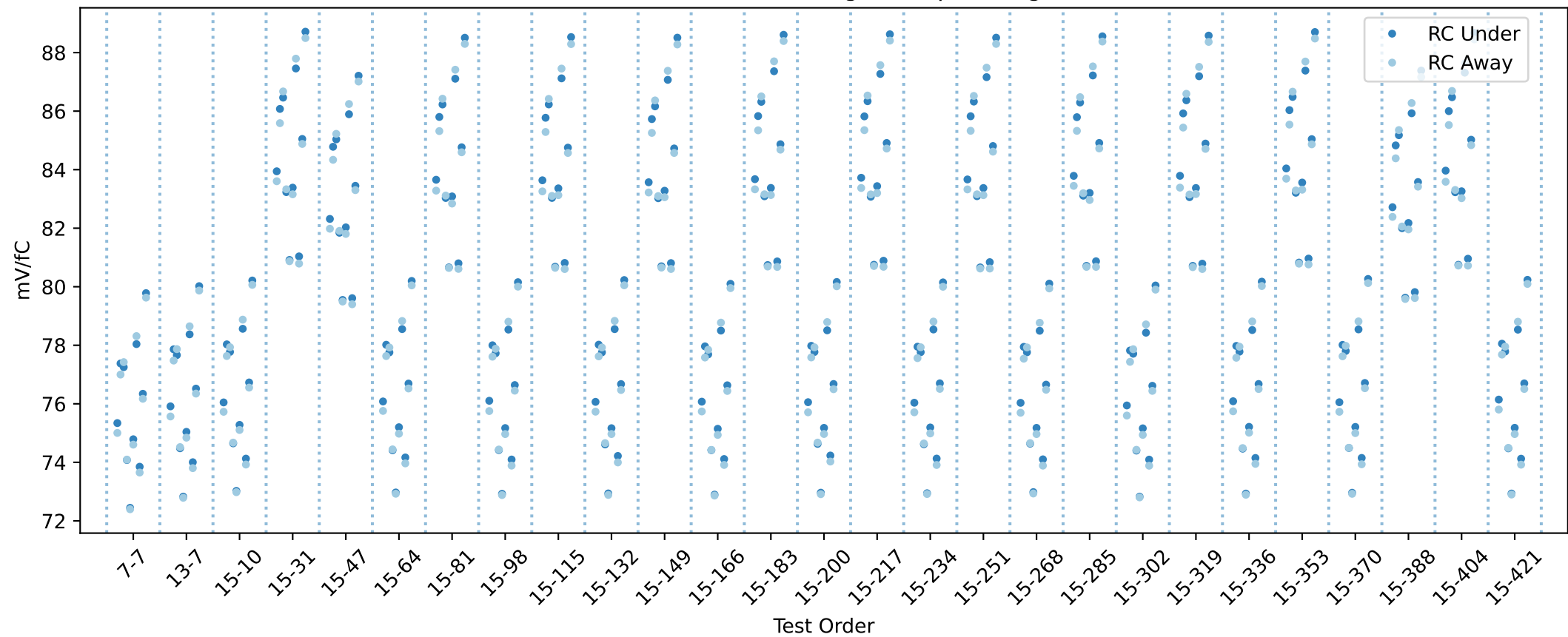
20USBHX2001943 RC gain chip averages
