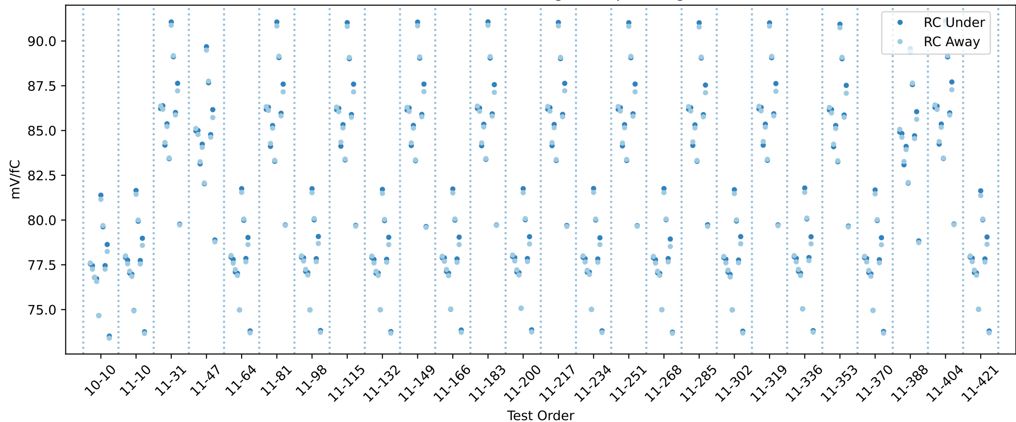
20USBHX2002025 RC gain chip averages
