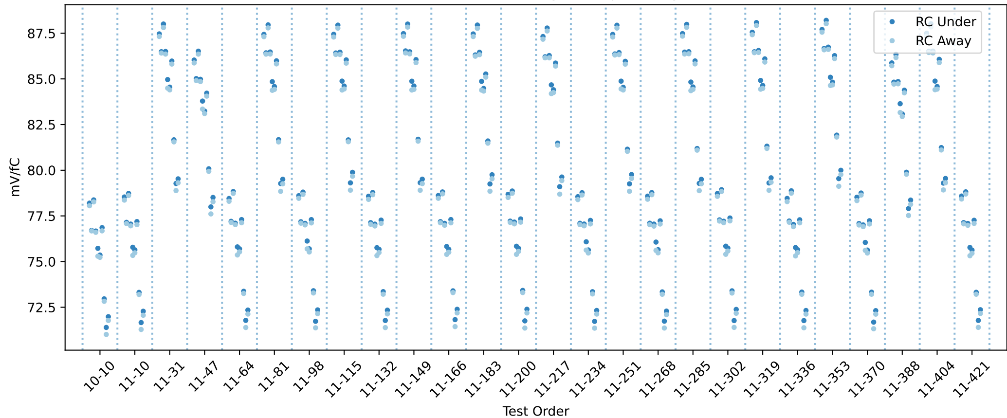
20USBHX2002027 RC gain chip averages
