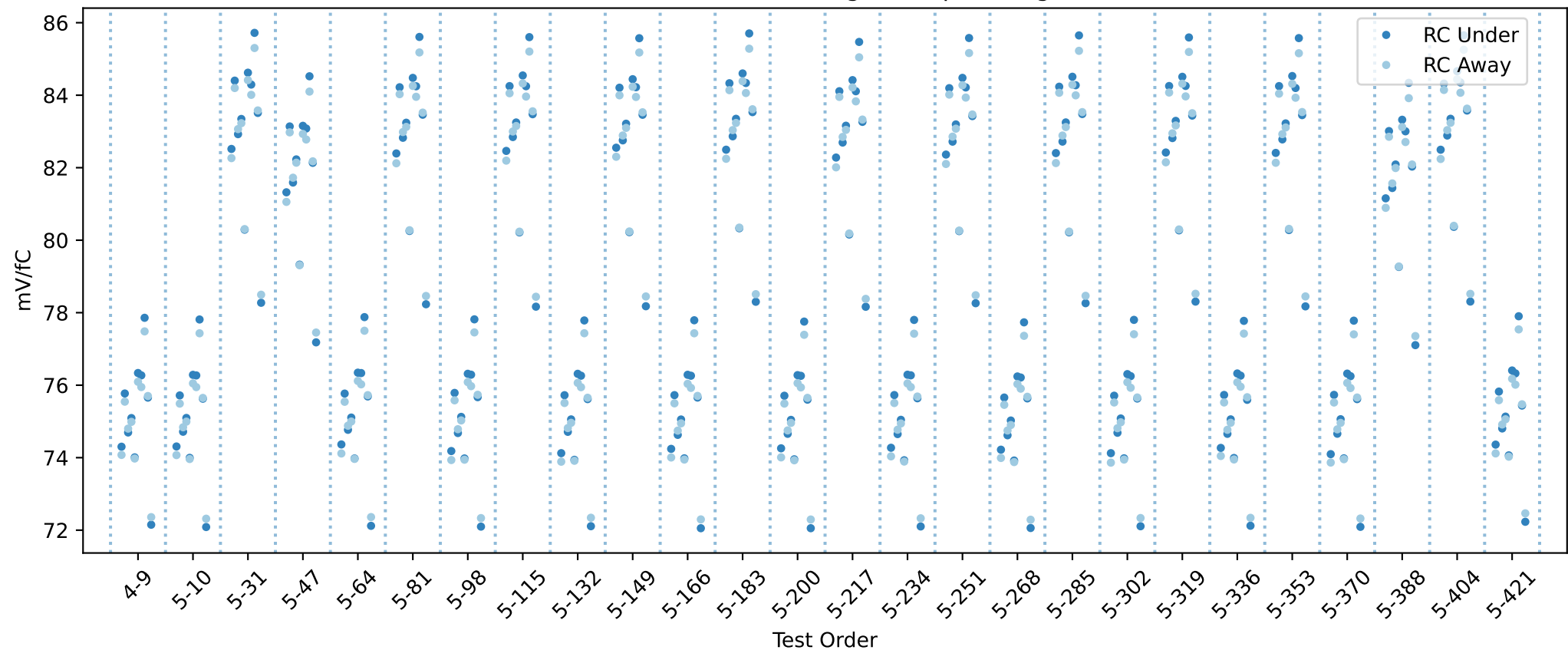
20USBHX2002030 RC gain chip averages
