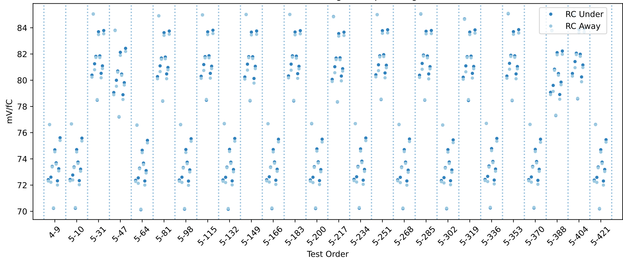
20USBHX2001987 RC gain chip averages
