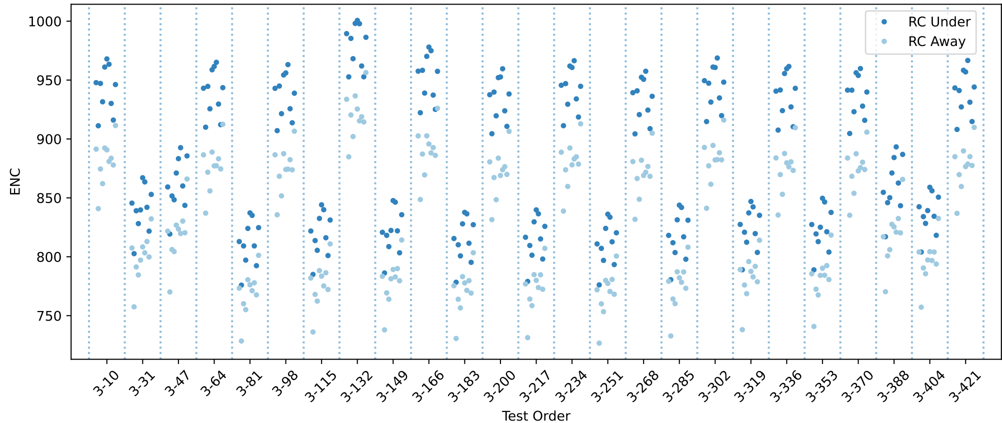
20USBHX2003752 RC innse chip averages
