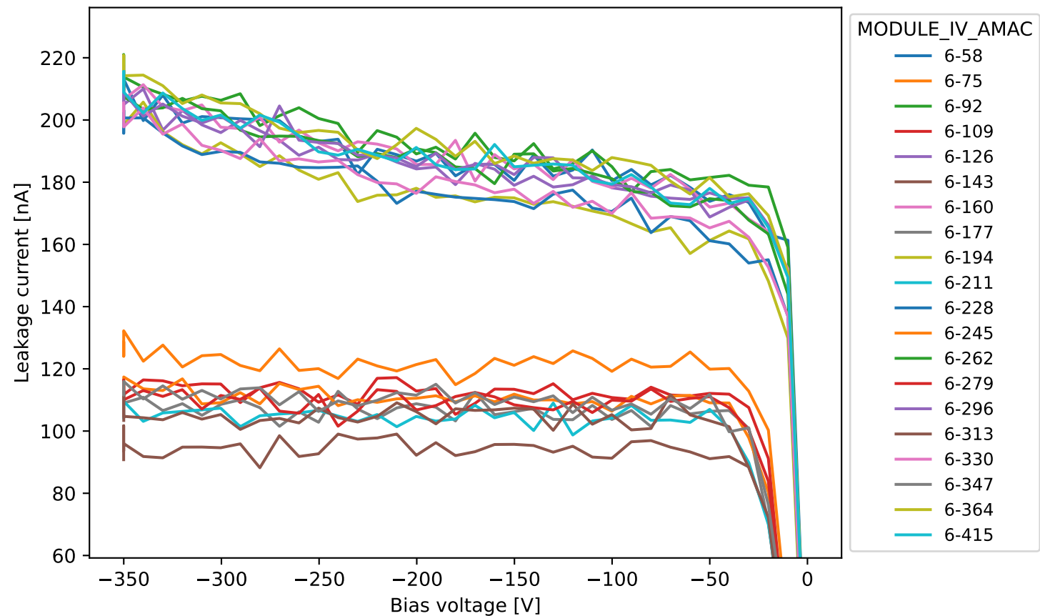
20USBML1236804 fast IV
