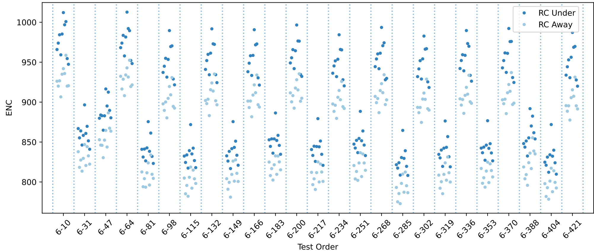
20USBHX2003746 RC innse chip averages
