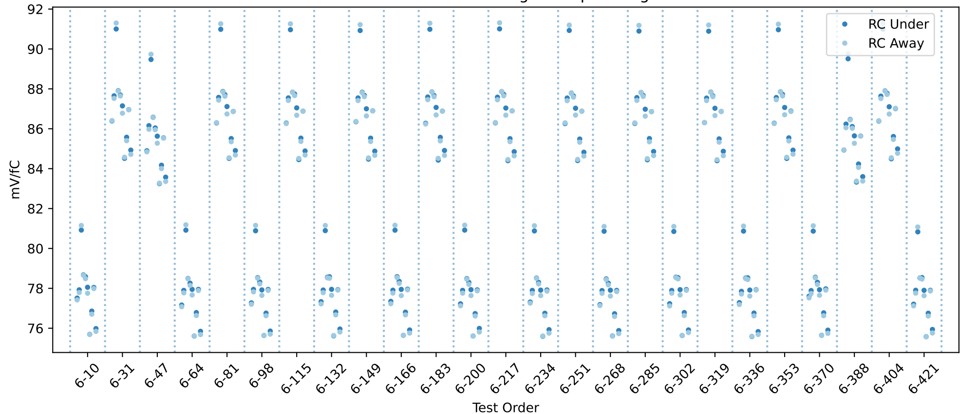
20USBHX2003747 RC gain chip averages
