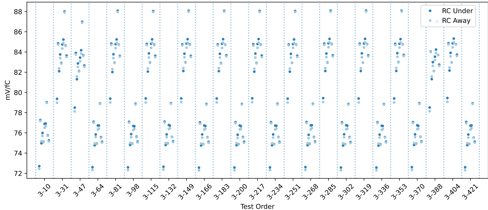
20USBHX2003451 RC gain chip averages
