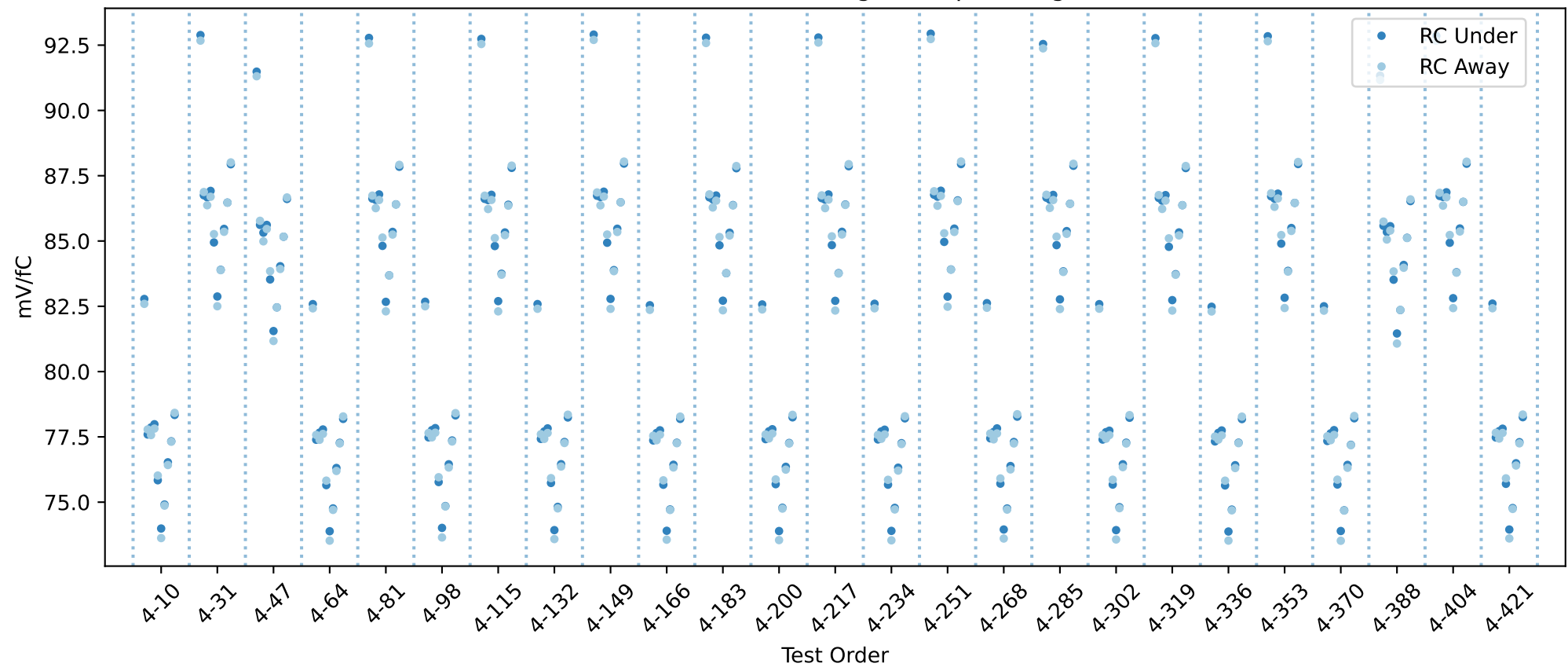
20USBHX2003474 RC gain chip averages
