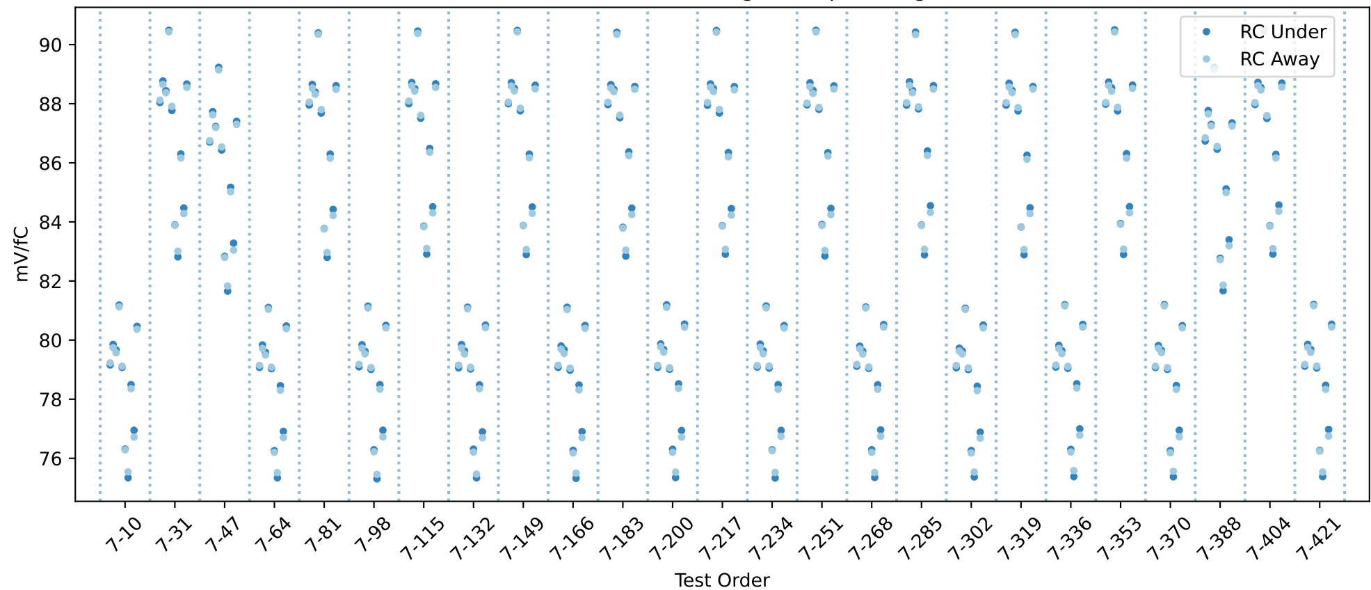
20USBHX2003781 RC gain chip averages
