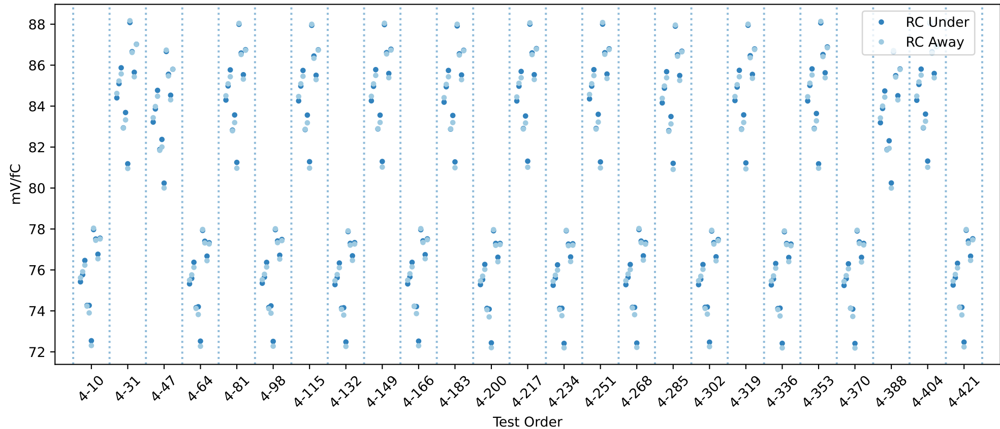
20USBHX2003789 RC gain chip averages
