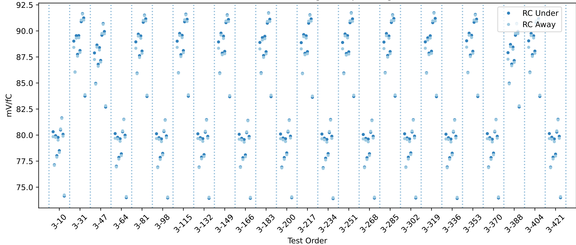
20USBHX2003784 RC gain chip averages
