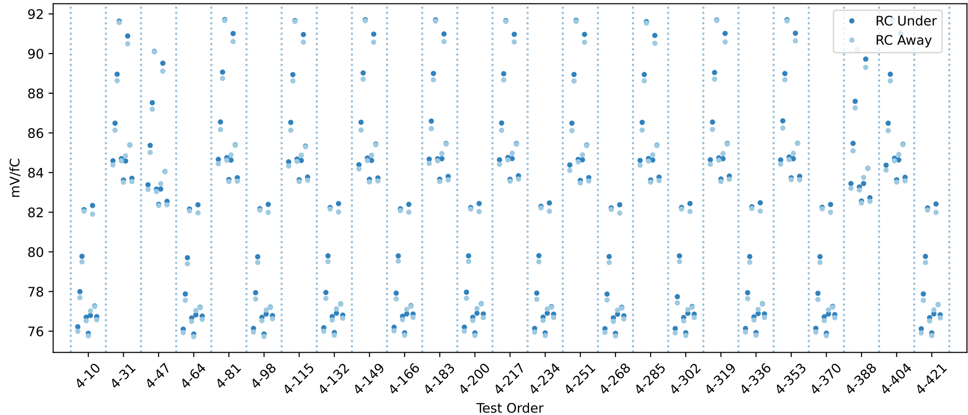
20USBHX2003785 RC gain chip averages
