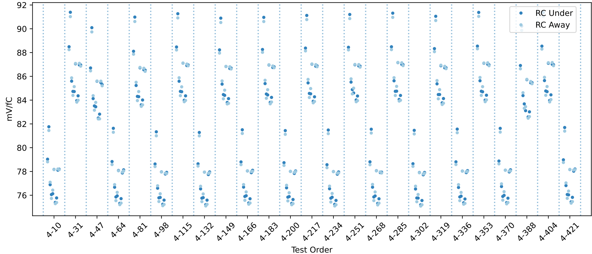
20USBHX2003786 RC gain chip averages
