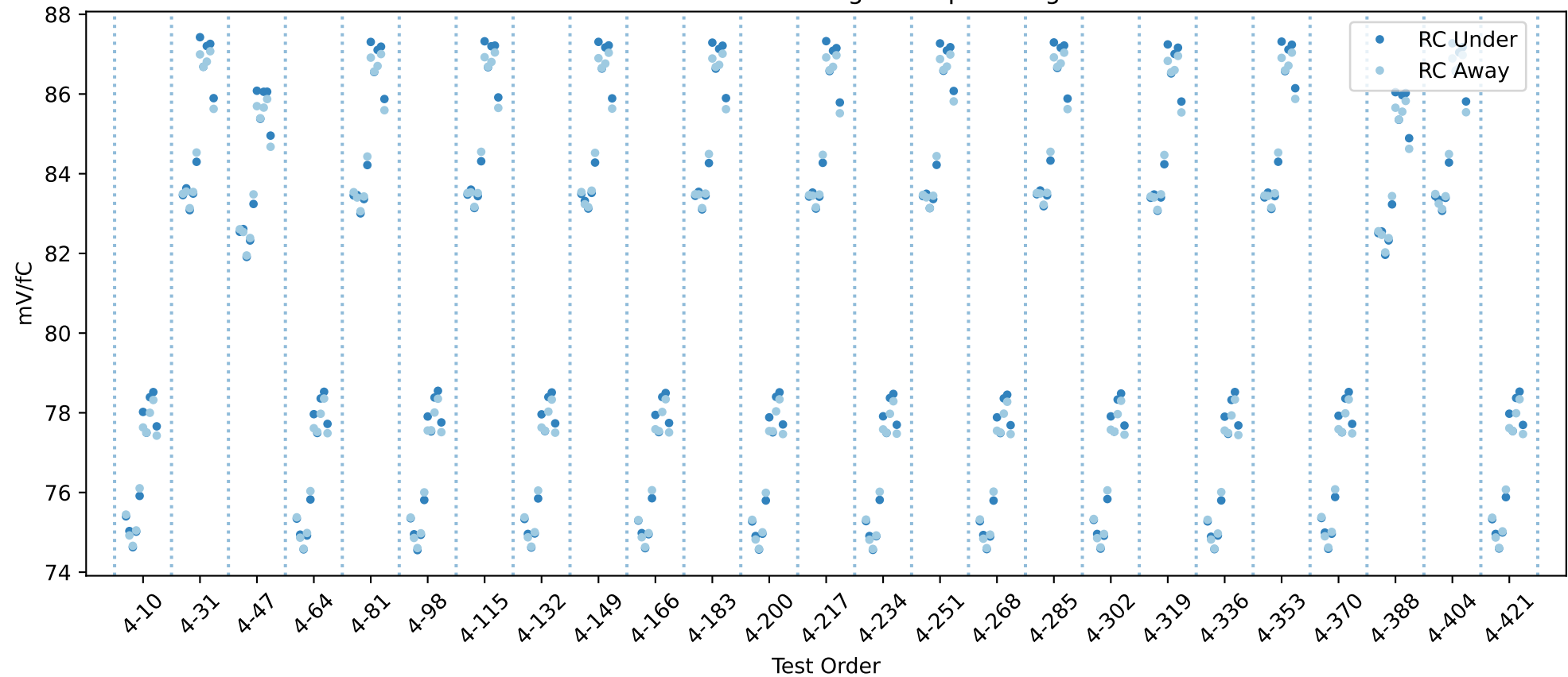
20USBHX2003793 RC gain chip averages
