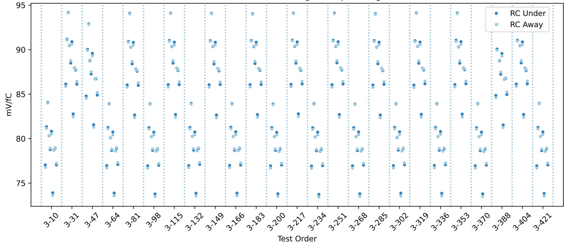
20USBHX2004263 RC gain chip averages
