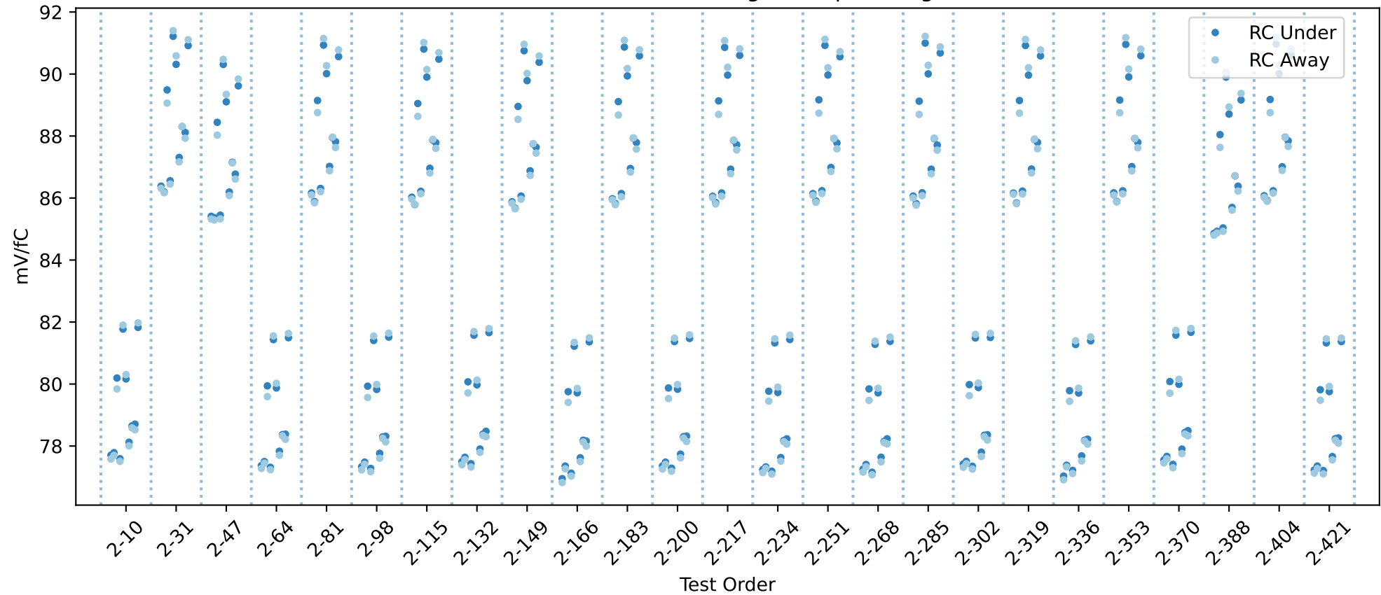
20USBHX2004236 RC gain chip averages
