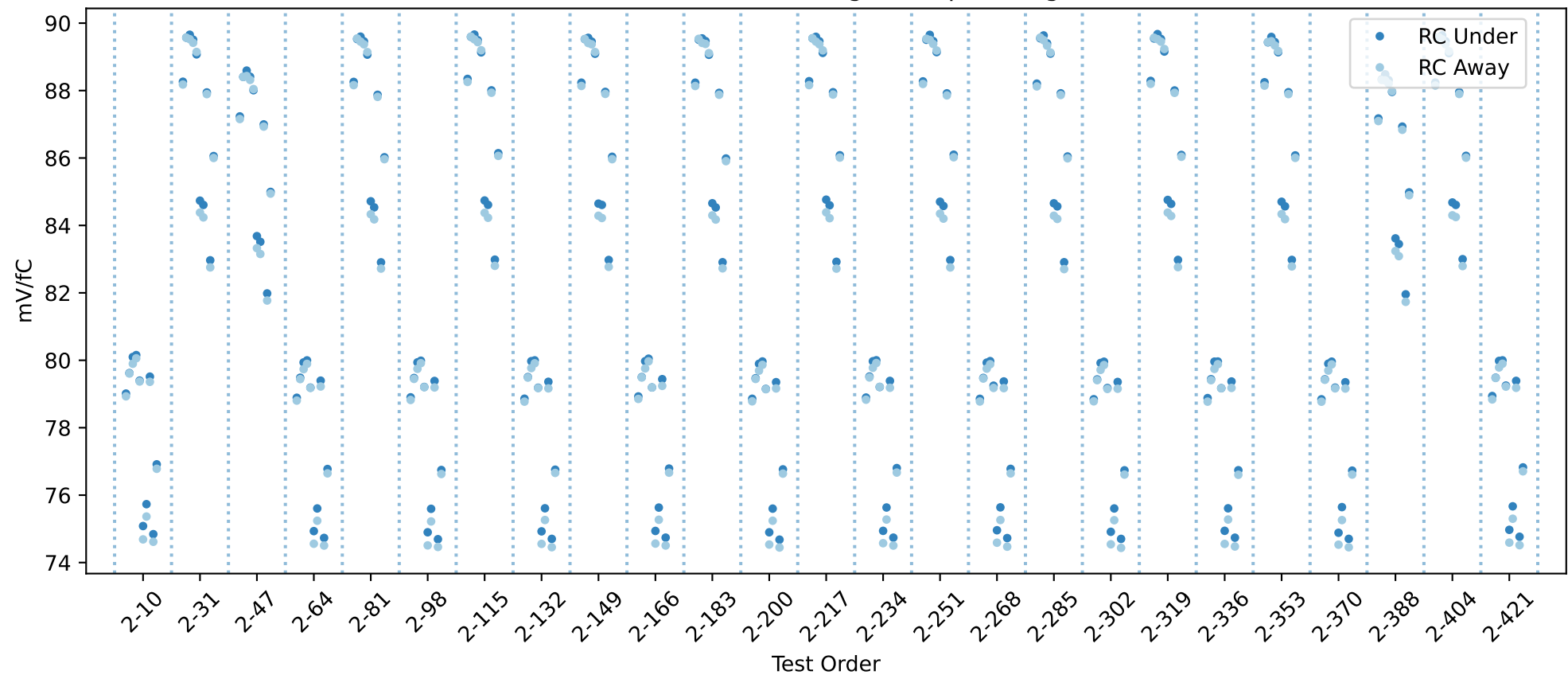
20USBHX2004237 RC gain chip averages
