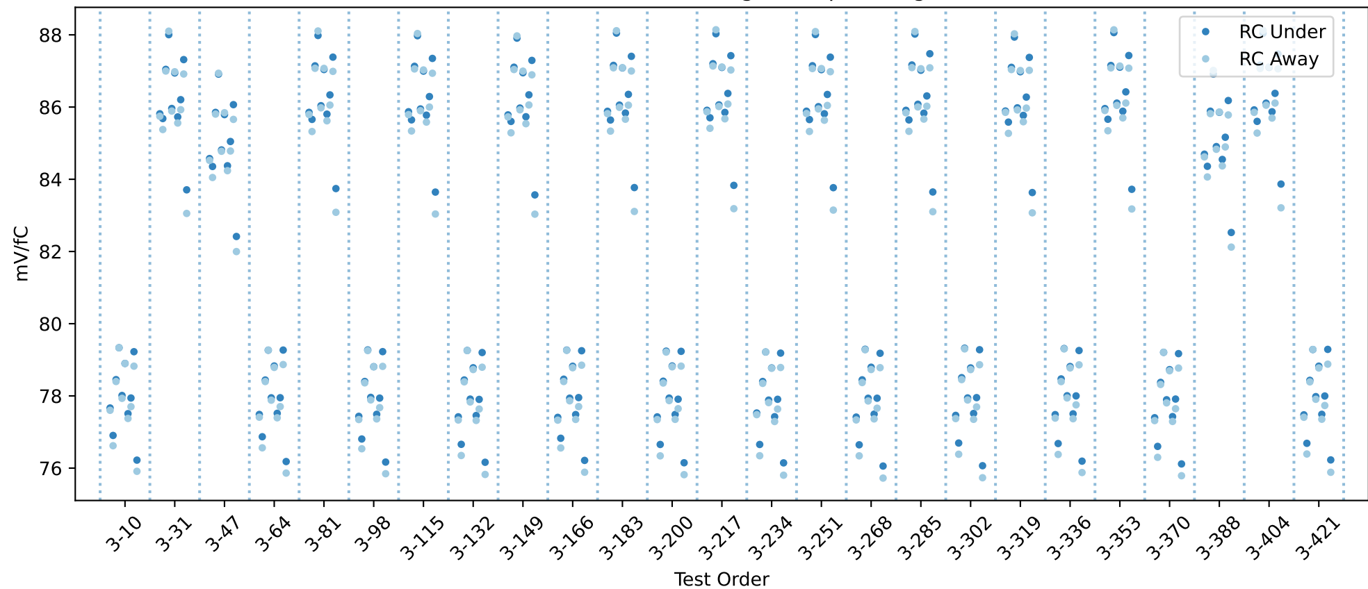
20USBHX2004239 RC gain chip averages
