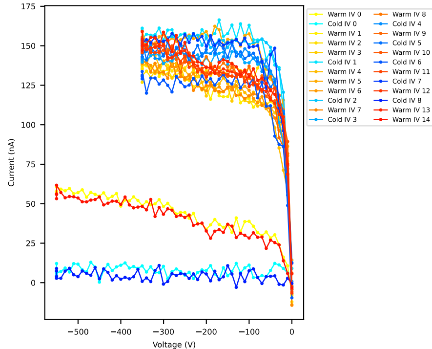
20USBML1237666 IV Results Throughout TC
