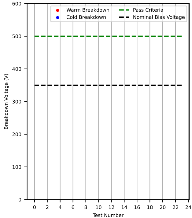
20USBML1237666 Breakdown Voltage Throughout TC
