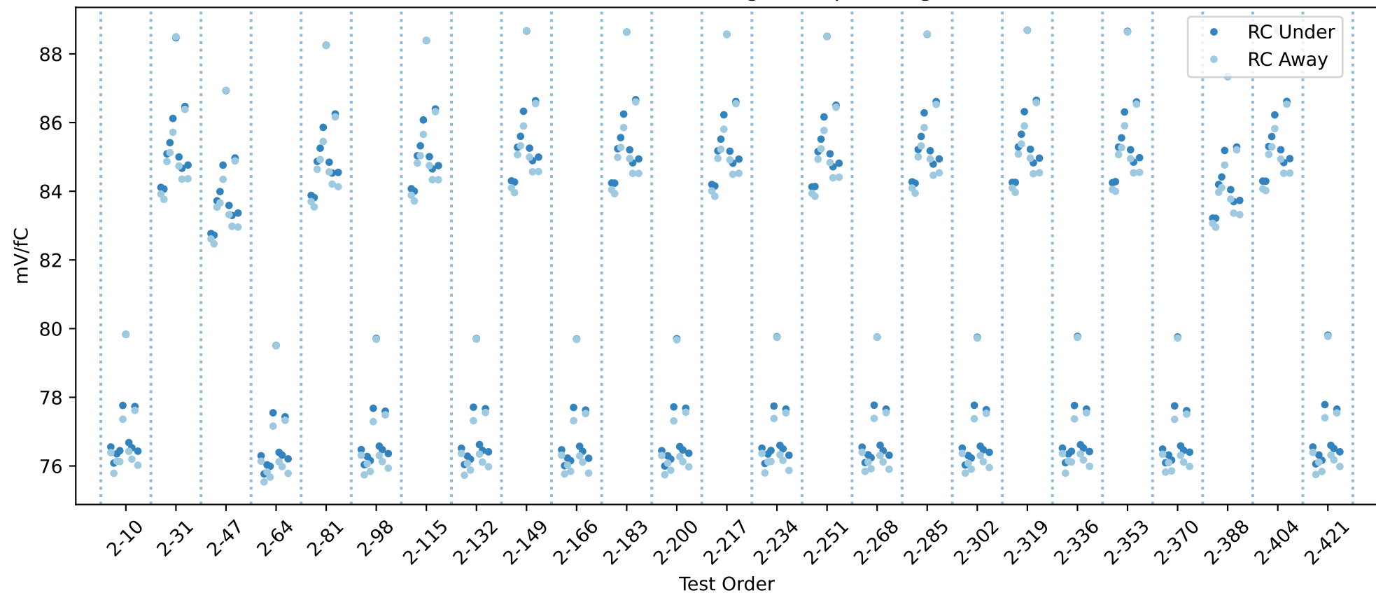
20USBHX2004244 RC gain chip averages
