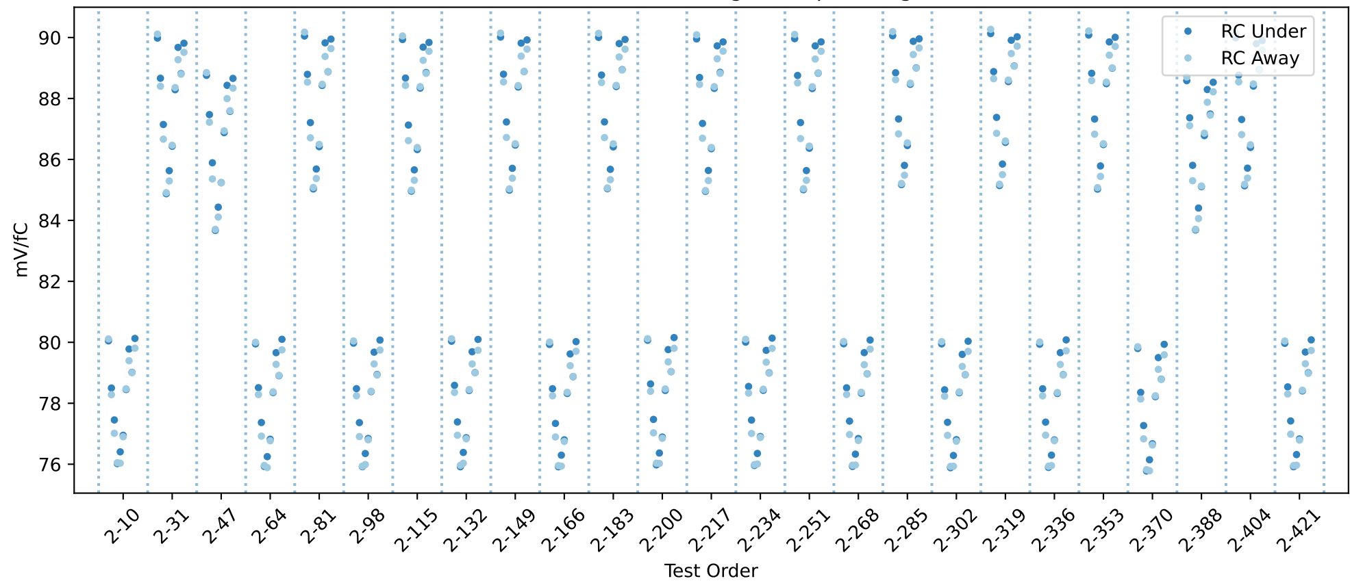
20USBHX2004544 RC gain chip averages
