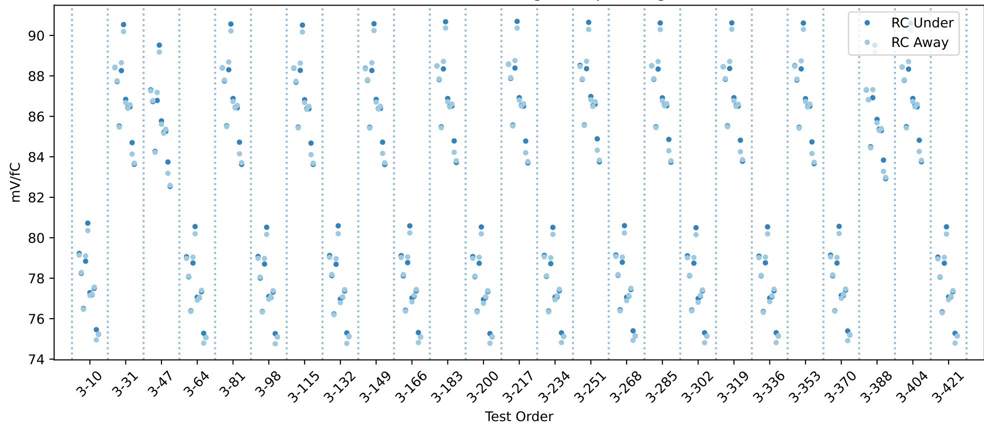
20USBHX2004547 RC gain chip averages
