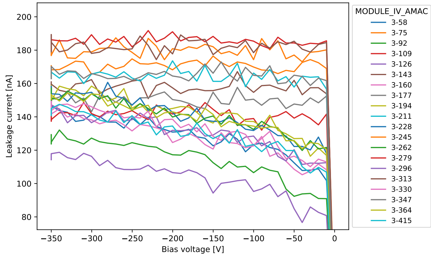
20USBML1237520 fast IV
