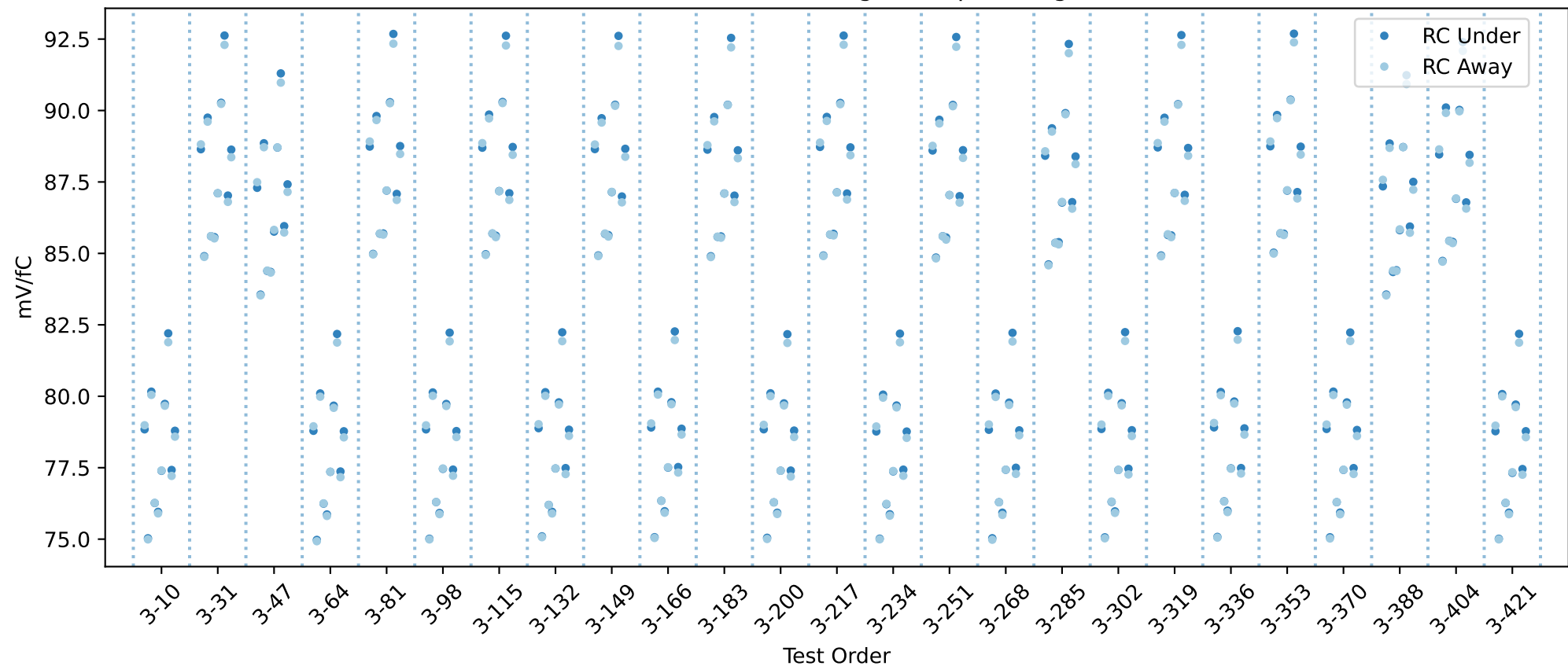
20USBHX2004548 RC gain chip averages
