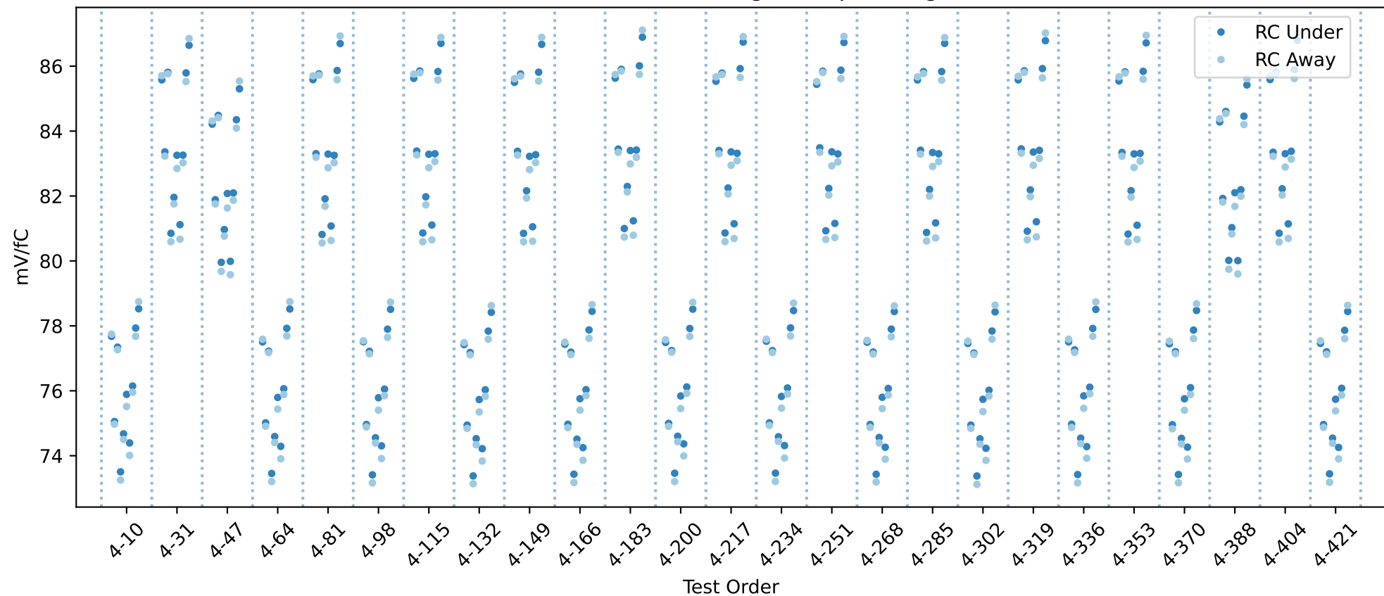
20USBHX2004666 RC gain chip averages
