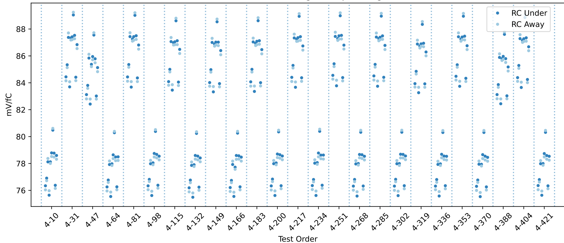
20USBHX2004667 RC gain chip averages
