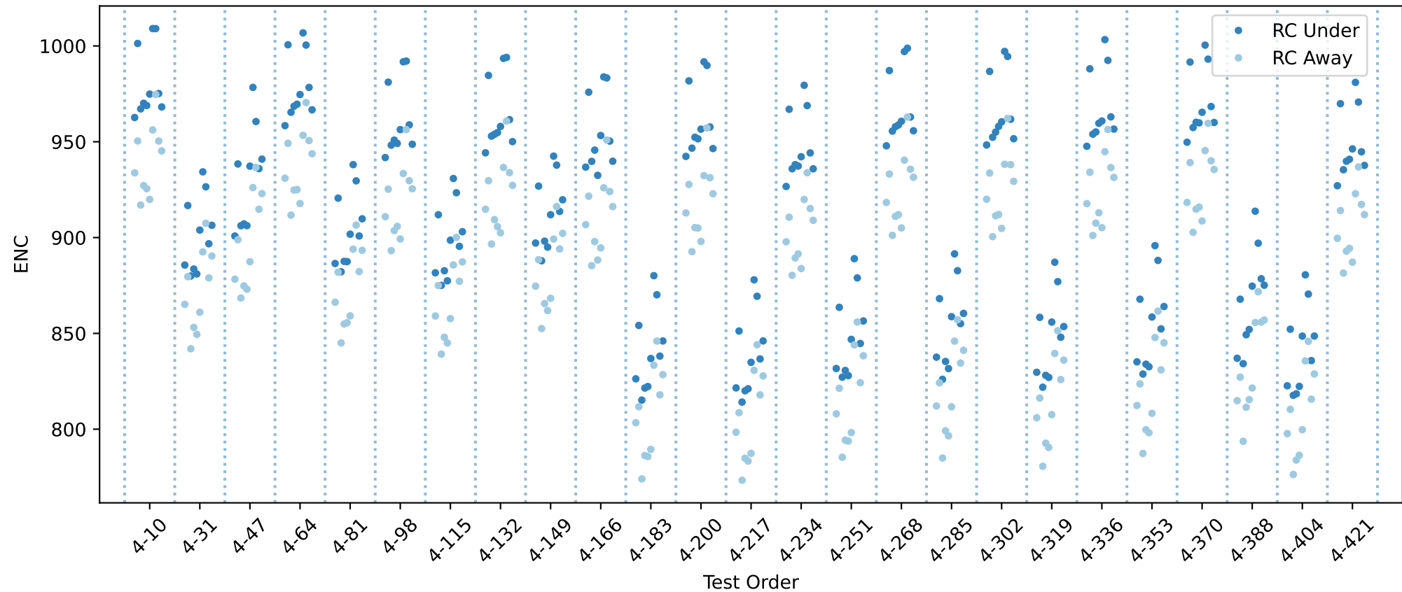
20USBHX2004667RC innse chip averages
