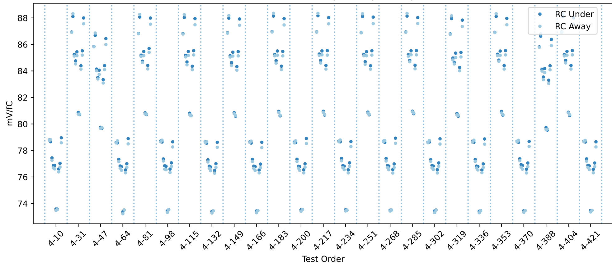
20USBHX2004668 RC gain chip averages
